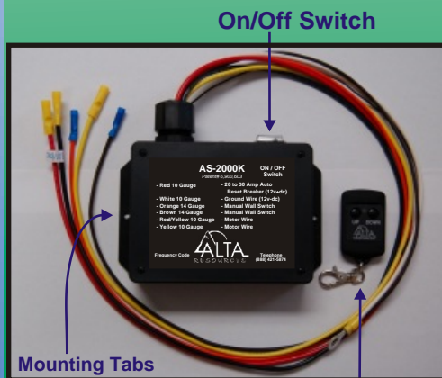
Wireless Remote Control Key Fob
